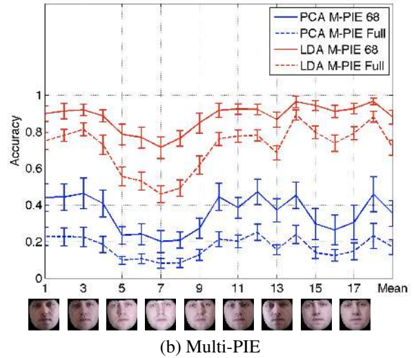
Figure 10. Comparison of PCA and LDA recognition across illumination conditions in PIE and Multi-PIE. For matched experimental conditions (PCA PIE 68 in (a) and PCA M-PIE 68 in (b)), performance is comparable, experimentally verifying the similarity in the physical setup of the two collections. Whereas LDA performance over PIE nearly saturates at 95%, the average accuracy over Multi-PIE using the largest test set (LDA M-PIE Full) indicates further room for improvement.
