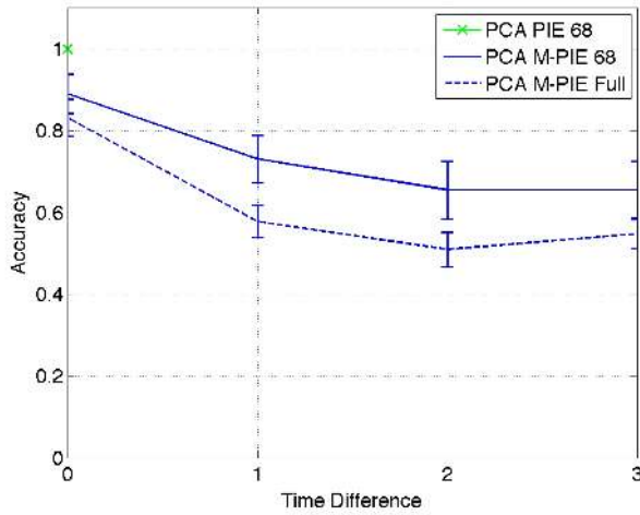
Figure 9. PCA performance for PIE and Multi-PIE across recording sessions. Since PIE only contains images from one session, gallery and probe images are identical, resulting in perfect recognition (PIE 68). For Multi-PIE, accuracies decrease with increasing time difference between the acquisition of gallery and probe images. We show results for a 68 subject subset of Multi-PIE (M-PIE 68) as well as for the full set of available subjects (M-PIE Full).
