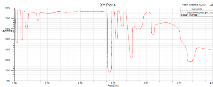
Fig 4. VSWR of Port B
