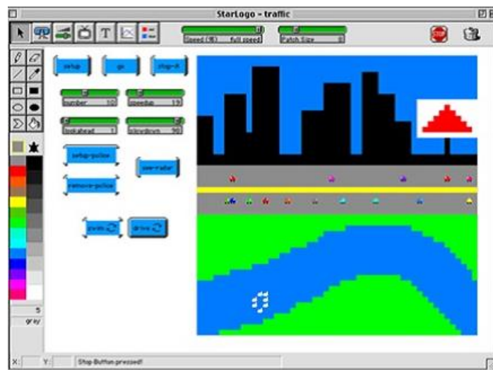
Figure 2. StarLOGO screenshot
