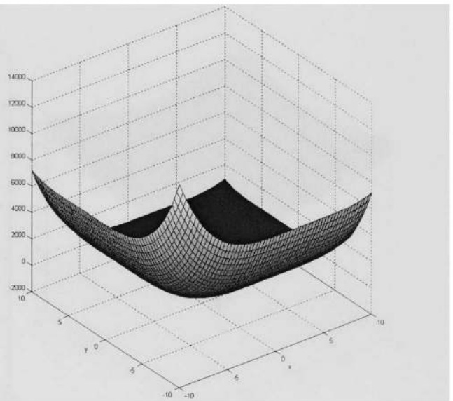
Figure 50: Rosen function
