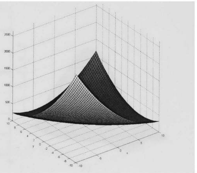
Figure 24: Booth function
