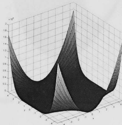
Figure 20: Beale function
