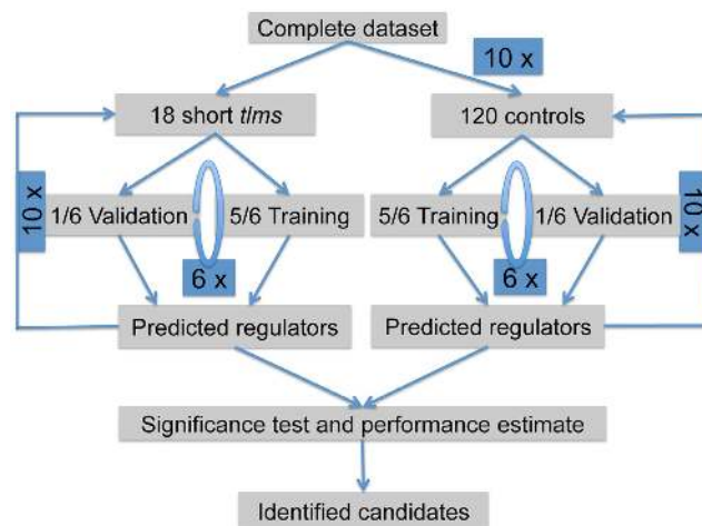
Figure 1. Schematic overview of the computational workflow. Using the expression profiles of short tlm knockout mutants as well as randomly selected control samples, a cross-validation was performed employing our linear modeling approach (inner loop for parameter optimization not shown). A significance test was performed to identify significant regulators being highly relevant for explaining expression of short tlm knockouts, while being not relevant for the controls.
