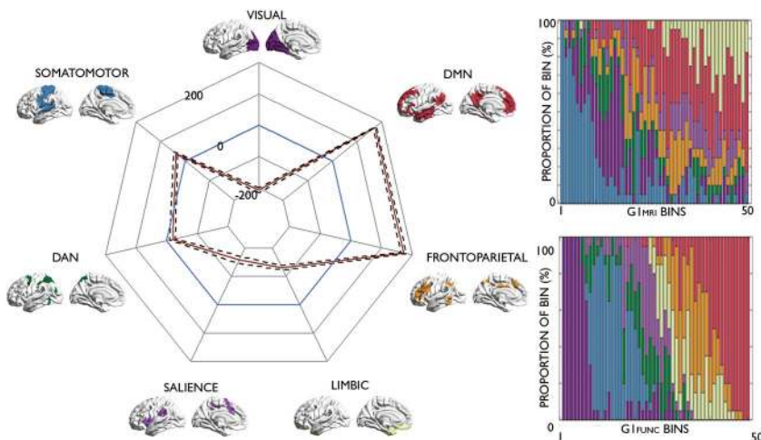
Fig 5. Divergent representations of the cortical hierarchy derived from microstructure and function. (A) Differences in nodal ranks between G1_{MRI} (blue) and G1_{FUNC} (red). (B) Radar plot depicting the difference in mean node ranks of functional communities [26] between G1_{MRI} (blue) and G1_{FUNC} (red), with 95% confidence intervals calculated across individuals presented with dotted lines; stacked bar plots depicting the proportion of each bin accounted for by intrinsic functional communities. (C) Meta-analysis maps for diverse cognitive terms were obtained from Neurosynth [28]. We calculated node-wise z-statistics, capturing node-term associations, and calculated the centre of gravity of each term along G1_{FUNC} and G1_{MRI} . The density plots depict the mean difference in the centre of gravity of meta-analysis maps in G1_{FUNC} and G1_{MRI} space across subjects. In vivo imaging data is openly available as part of the HCP S900 release ( https://www.humanconnectome.org/study/hcp-young-adult/document/900-subjects-data-release ). FUNC, functional; GI, first principal gradient; HCP, Human Connectome Project; MPC, microstructure profile covariance; MRI, magnetic resonance imaging.
