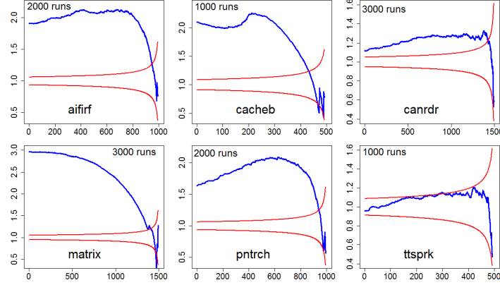
Fig. 12. CV-plot for aifirf, cacheb, canrdr, matrix, pntrch and ttsprk.
