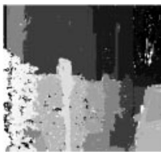
GPM-MRF results
