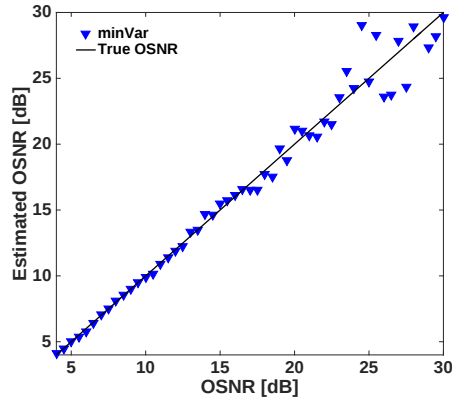
Fig. 7. OSNR estimation using minimum variance feature with trained NN for DP-64 QAM and RC 0.01 pulseshaping.
