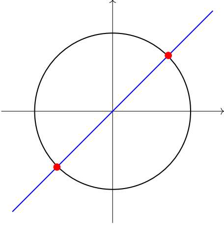
Figure 1. For every vector \mathbf{h} \in \mathbb{R}^2 \setminus \{0\} , the linear subspace \mathcal{T}_{\mathbf{h}} := \{\mathbf{h}z : z \in \mathbb{R}\} intersects the unit circle S_1 in the two antipodal points \pm \mathbf{h}/\|\mathbf{h}\|_2 .
