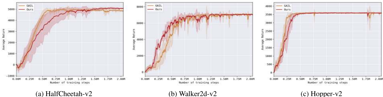
Figure 8. Learning curves for primitive tasks. The darker-colored lines and shaded areas denote the average returns and standard deviations, respectively, computed over 10 random seeds. These graphs indicate that our method can successfully learn primitive tasks.
