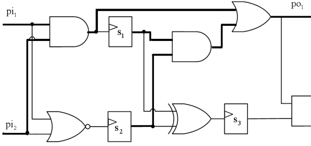
Fig. 1. Example circuit
