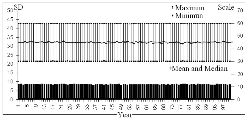
Figure 4: Evolution of propensity to remit wages Rw in 100 years.
