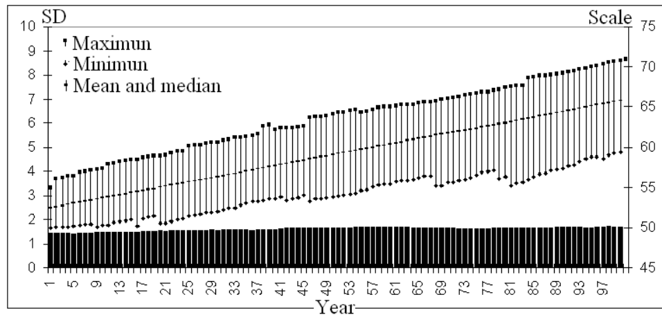
Figure 2: Evolution of networks S_n in 100 years.
