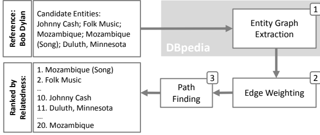
Figure 2: Entity ranking workflow.
