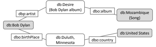
Figure 3: Example of multiple paths between entities with different semantic specificity.
