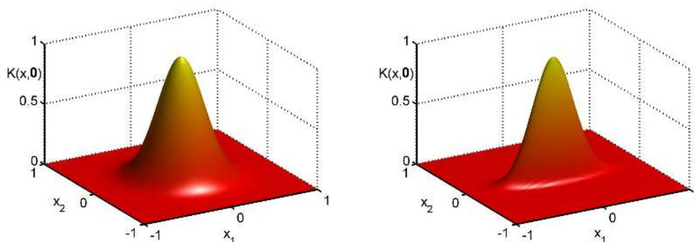
(a) Isotropic Gaussian kernel with shape parameter \varepsilon = 3 .
