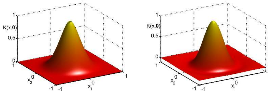
(a) C^2 Wendland function \kappa(r) = (1-r)_+^4(4r+1) centered at the origin in \mathbb{R}^2 . (b) \kappa(r) = (1 - \varepsilon^2 r^2 + \frac{\varepsilon^4 r^4}{6})e^{-\varepsilon^2 r^2} , a Laguerre-Gaussian kernel with \varepsilon = 3 centered at the origin in \mathbb{R}^2 .
