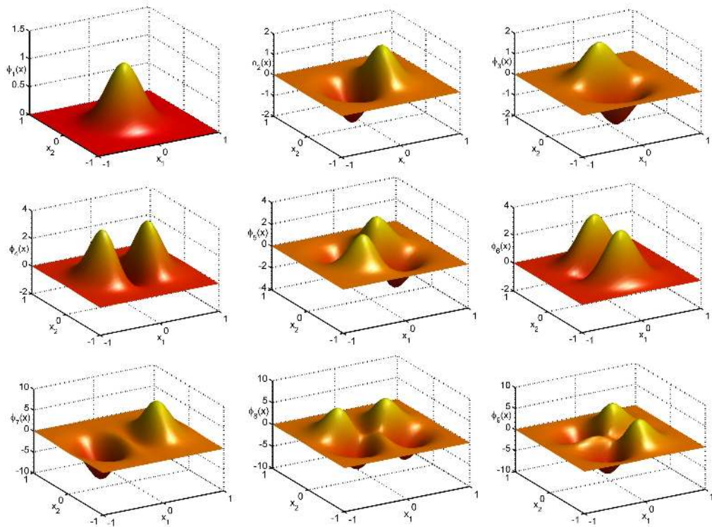
Figure 25: The first few Gaussian eigenfunctions for \varepsilon = 3 and \alpha = 6 .
