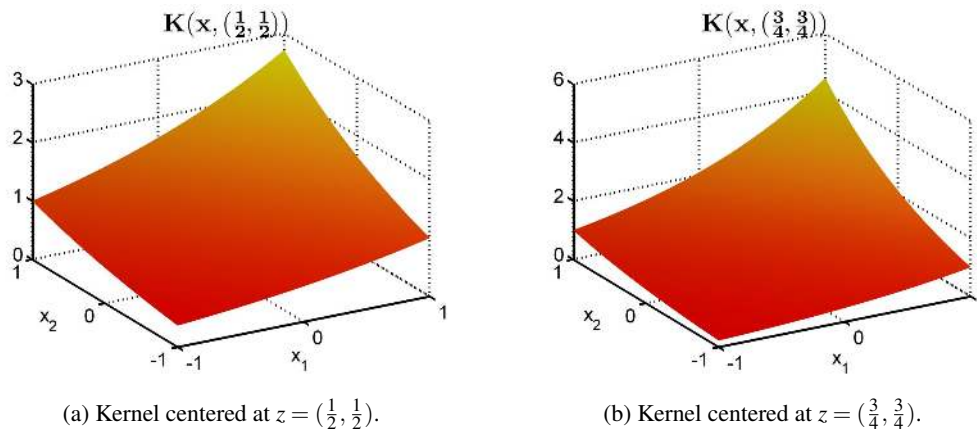
Figure 11: Exponential power series kernels.
