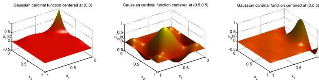
Figure 18: Gaussian cardinal basis functions centered at different points in the unit square.
