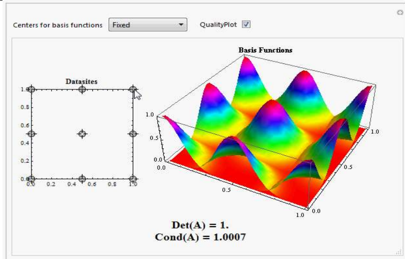
Figure 16: Screen shot of the Mathematica module used to illustrate the proof and implications of the Mairhuber-Curtis theorem.
