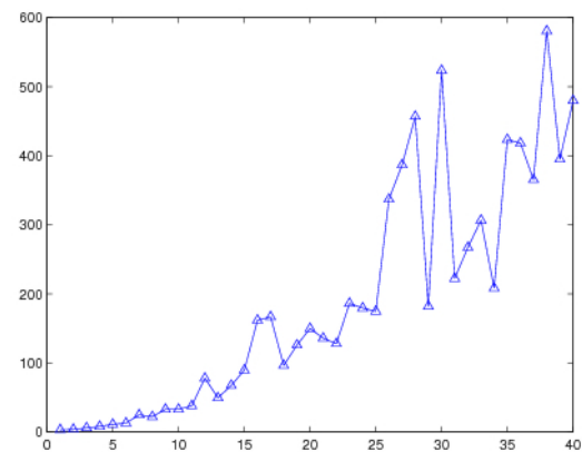
Figure 1: Left: N = 861 Discrete Leja Points for degree n = 40 on the square, extracted from an 81 \times 81 Chebyshev-Lobatto grid; Right: Lebesgue constants of Discrete Leja Points on the square for n = 1, \dots, 40 .
