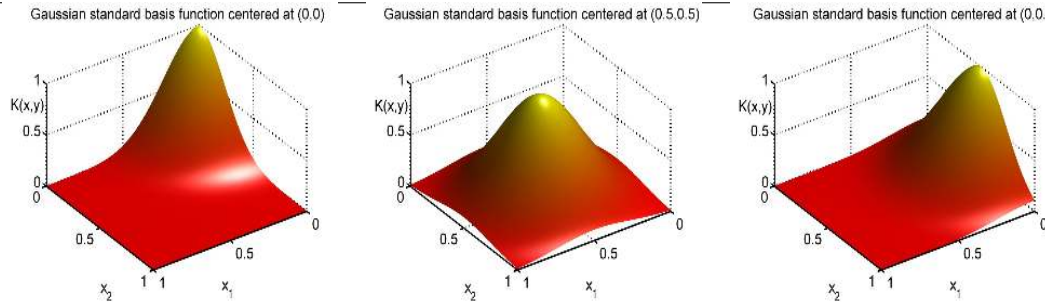
Figure 17: Standard Gaussian basis functions centered at different points in the unit square.
