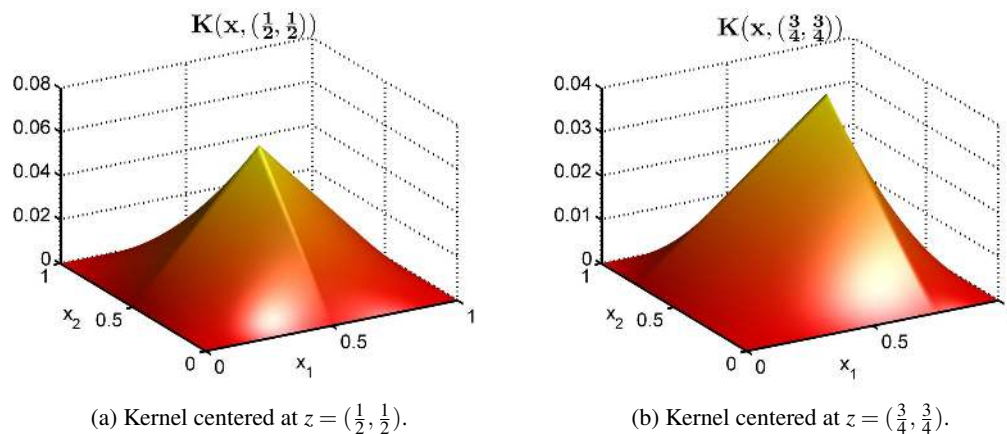
Figure 12: Brownian bridge tensor product kernels.
