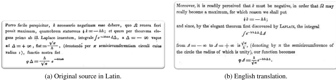
Figure 4: Excerpt from [57, Sect.177] showing the first occurrence of the Gaussian kernel in the work of Gauß.
