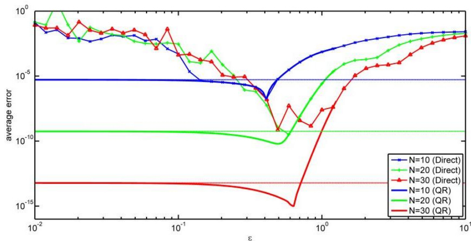
Figure 26: Illustration of spectral accuracy achievable with the RBF-QR interpolation algorithm on Chebyshev points.
