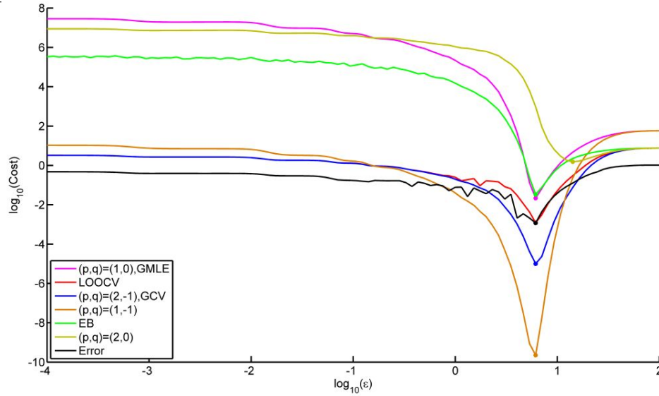
Figure 22: Comparison of different criteria to select an “optimal” shape parameter \varepsilon in Gaussian kernel interpolation.
