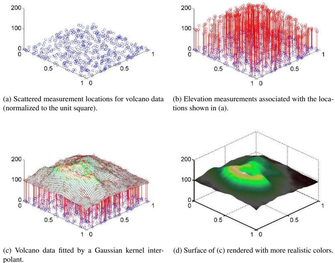
Figure 14: Illustration of the scattered data fitting problem.
