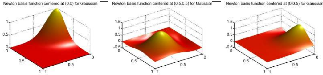
Figure 19: Gaussian Newton-type basis functions centered at different points in the unit square.
