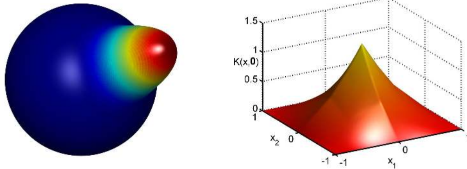
(a) Spherical Gaussian with shape parameter \varepsilon = 9 and z = \frac{1}{\sqrt{3}}(1, 1, 1) . (b) Piecewise linear multiscale kernel centered at z = (0, 0) .
