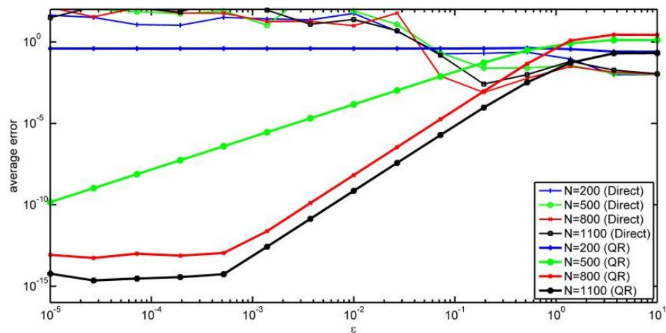
Figure 27: High-accuracy approximation of a 5D polynomial using the RBF-QRr approximation algorithm on Halton points.
