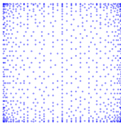
Figure 1: Left: N = 861 Discrete Leja Points for degree n = 40 on the square, extracted from an 81 \times 81 Chebyshev-Lobatto grid; Right: Lebesgue constants of Discrete Leja Points on the square for n = 1, \dots, 40 .
