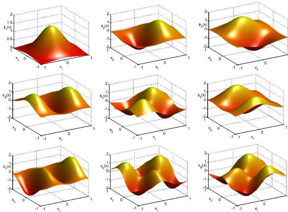
Figure 24: The first few Gaussian eigenfunctions for \varepsilon = 3 and \alpha = 1 .
