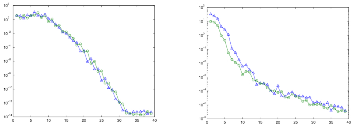
Figure 2: Uniform error (circles) and estimate (2.7) (triangles) of Newton interpolation at Discrete Leja Points on the square for v = 2, \dots, 40 ; Left: f(x_1, x_2) = \cos(5(x_1 + x_2)) ; Right: f(x_1, x_2) = [(x_1 - 1/3)^2 + (x_2 - 1/3)^2]^{5/2} .
