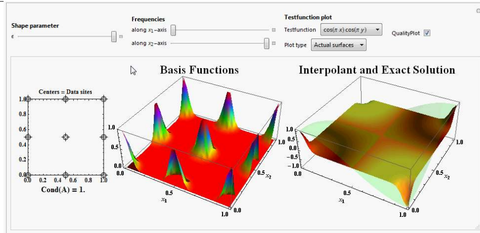
Figure 21: Screen shot of the Mathematica module used to illustrate effects of the Gaussian shape parameter.
