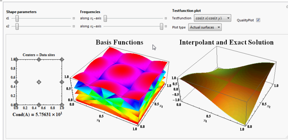
Figure 23: Screen shot of the Mathematica module used to illustrate anisotropic Gaussian interpolation.
