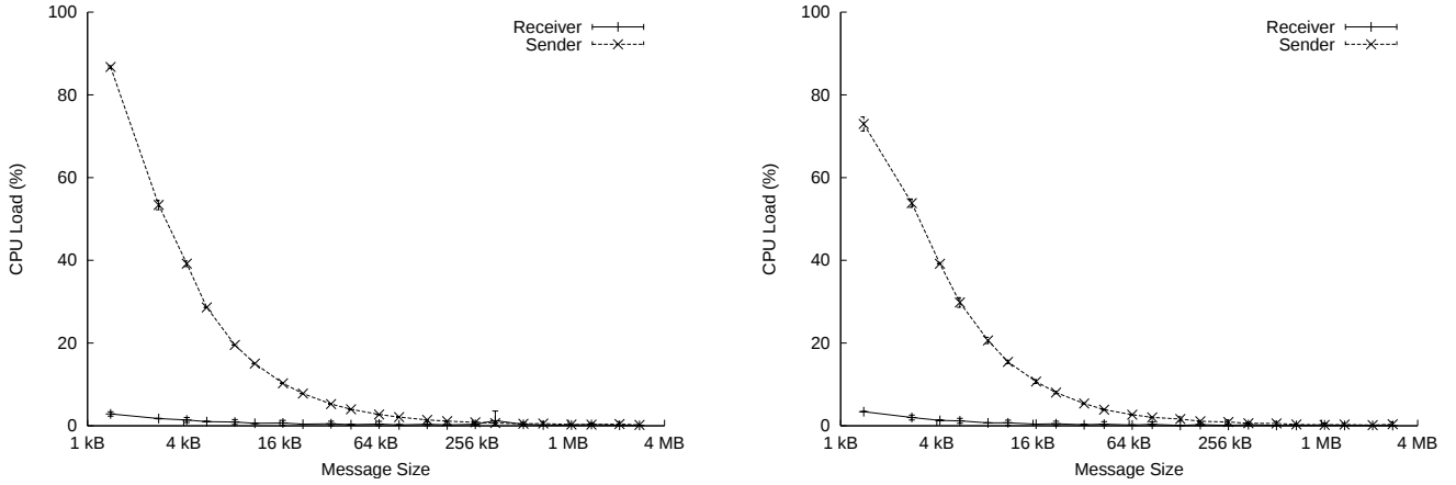
Figure 3. Host CPU utilization for a node using the hardware iWarp stack when connected to a peer with either (a) hardware or (b) software iWarp stack.
