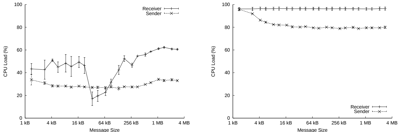
Figure 4. (a) Host CPU utilization, both nodes using TCP, not iWarp. (b) Host CPU utilization for a node using the software iWarp stack when connected to a peer using the hardware iWarp stack.
