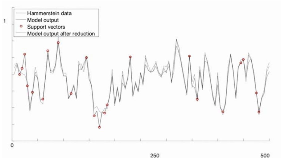
Figure 3. Identified Hammerstein System, support vectors and model output after reduction
