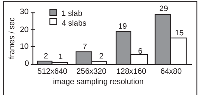
Fig. 6. Performance of the compositing-splatting-display back-end, measured with by-passed image generation code in the ray casting nodes. These numbers are independent of the number of computing nodes present in the system.
