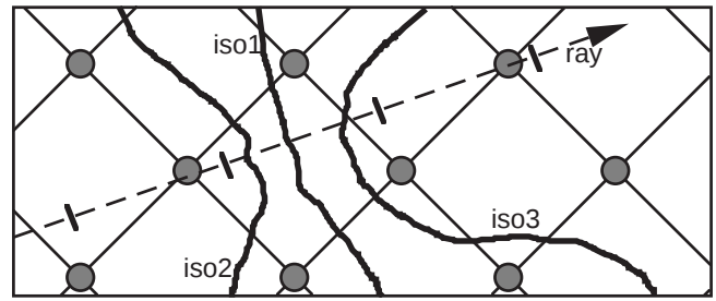
Fig. 10. Isosurfaces between samples along a ray are encountered in algorithmic order but must be sorted for compositing. Surfaces detected in \langle 1,2,3 \rangle -order must be composited in \langle 2,1,3 \rangle -order.
