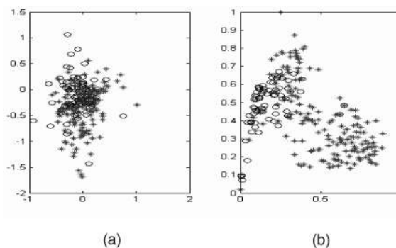
Fig. 6. Data distribution in the projected subspace: (a) DEM and (b) KDEM. Different samples are more separated and clustered in the nonlinear subspace by KDEM (*: class Cytoplasmic ribosome, o: class Proteasome).
