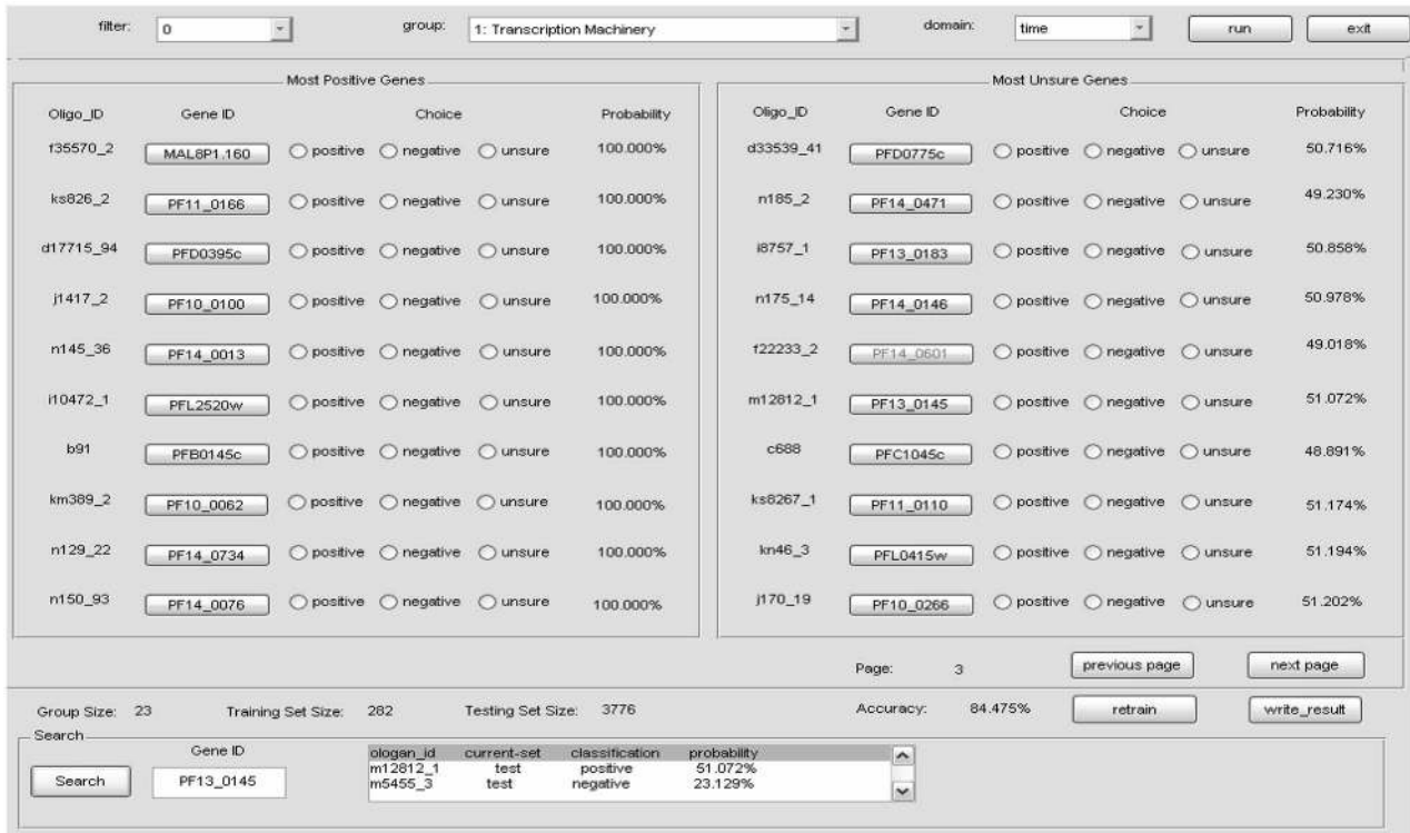
Fig. 8. The interactive semisupervised learning system for gene classification and retrieval.
