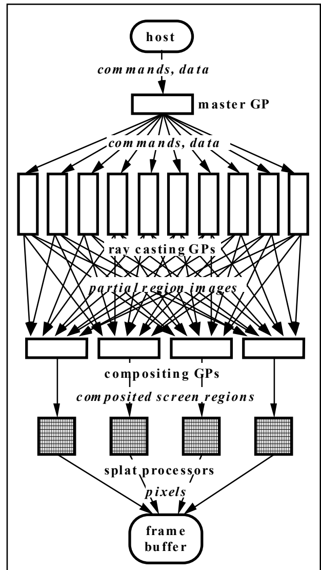
Fig. 5 - Visualization pipeline
