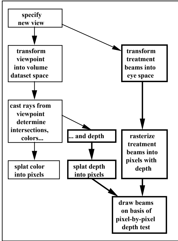
Fig. 10 - Algorithm for adding line primitives
