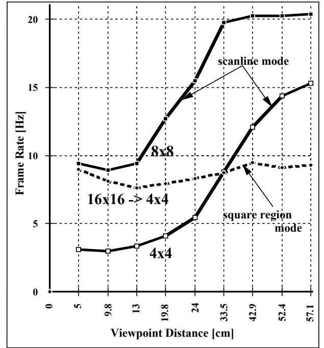
Fig. 12 - Frame rate comparison between line and square region partitions for varying object size. (Full screen images are produced by 5 cm viewpoint distance, 60 cm distance produces 1/16 screen coverage.) Line partitions cast rays every 8x8 or 4x4 pixels. Square regions are adaptively sampled initially at one ray per 16x16 pixels and refined up to one ray per 4x4 pixels.
