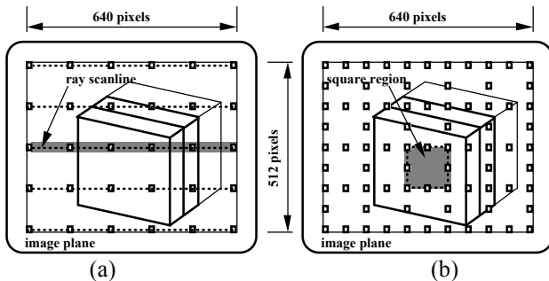
Fig. 11 - Image space partitioning by a)lines and b)square regions
