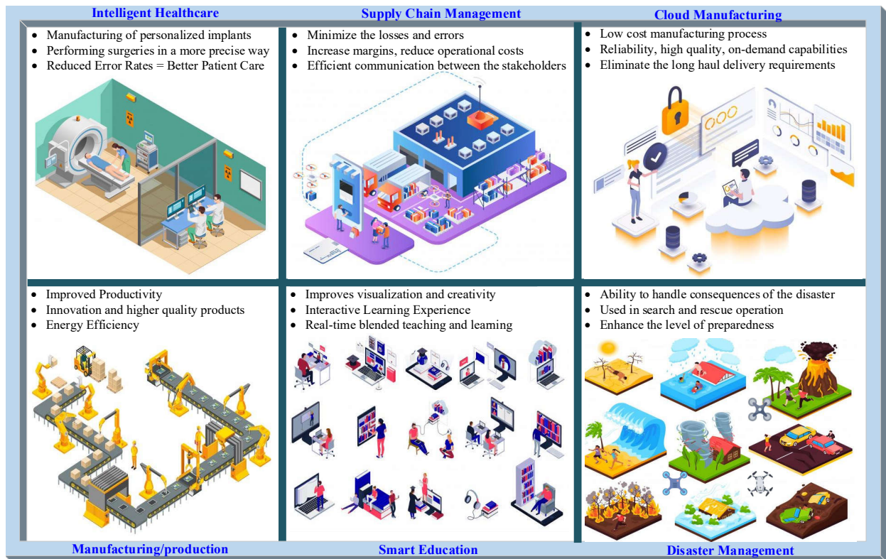
Figure 2: Industry 5.0 applications.
