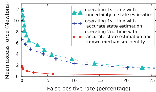
Fig. 12 Effect of errors in kinematic state estimation on performance of anomalous force detection using data captured with Cody and the PR2
