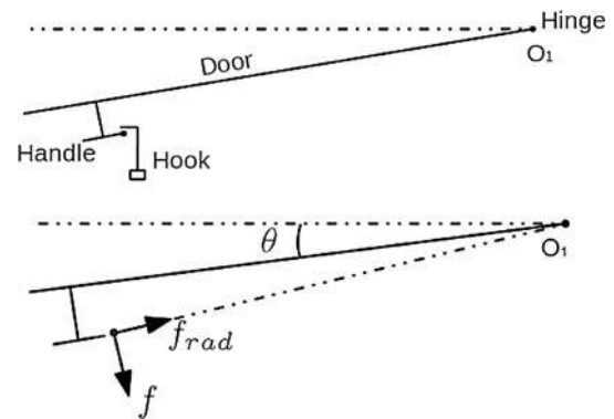
Fig. 2 Top: Diagram showing the top view of a door as it is opened using a hook. Bottom: The relevant force, f , is the component of the total force between the hook and the handle that is tangential to the trajectory of the point of contact on the door handle. We refer to this component as the opening force. The radial force, f_{rad} , will result in constraint forces at the hinge. The relevant mechanism state is the opening angle, \theta
