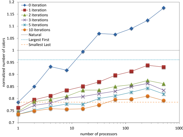
Figure 7. Impact of the number of iterations on real-world graphs in distributed memory
