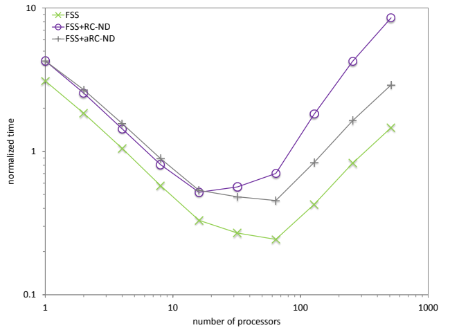
Figure 6. Comparison of recoloring on real-world graphs with Smallest Last ordering
