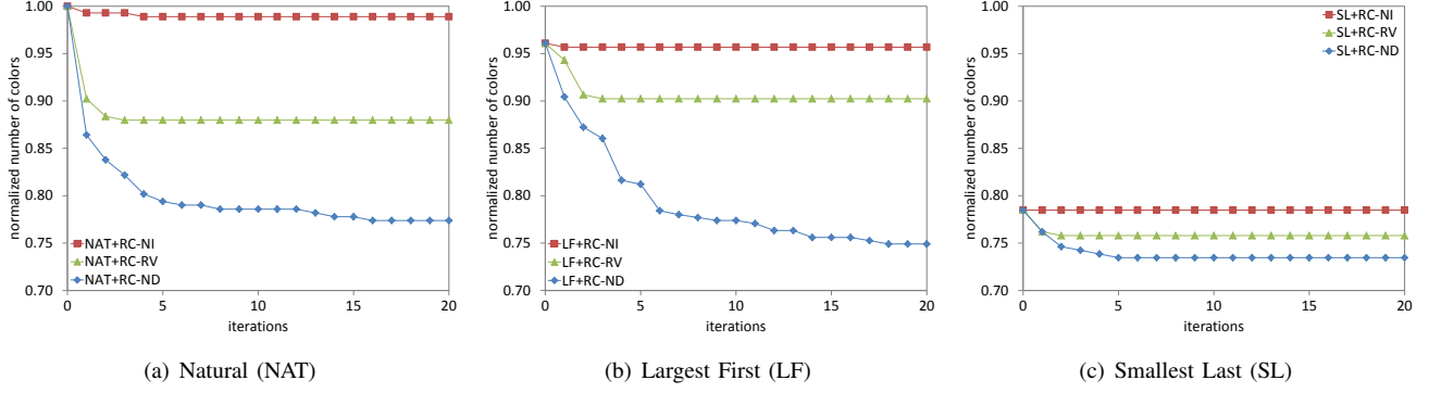
Figure 1. Sequential study on the real graphs
