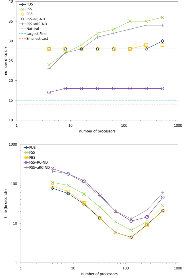
Figure 4. Comparison of ordering and recoloring on RMAT-Good
