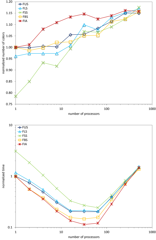
Figure 2. Comparison of ordering on the real graphs
