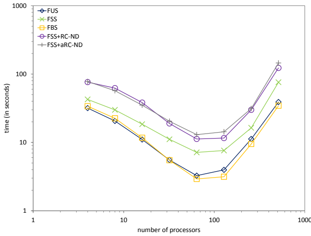
Figure 5. Comparison of ordering and recoloring on RMAT-Bad
