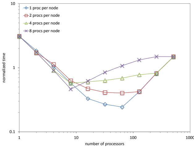
Figure 8. Impact of the processor allocation policy on real-world graphs in distributed memory
