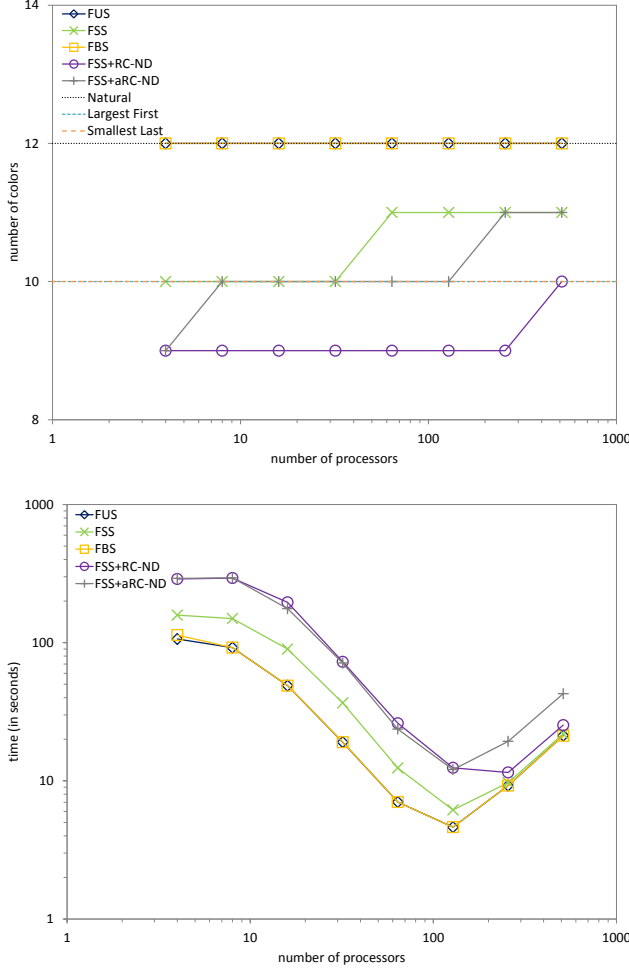
Figure 3. Comparison of ordering and recoloring on RMAT-ER
