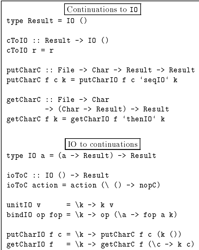
Figure 2: Converting between continuations and IO
