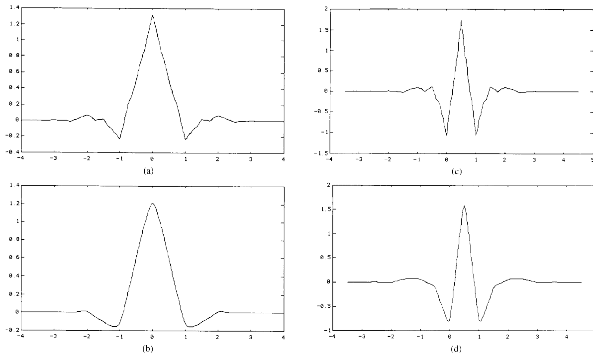
Fig. 3. Scaling functions \phi, \tilde{\phi} and wavelets \psi, \tilde{\psi} for example 2 (spline variant with less dissimilar lengths: l = 4 = k, \tilde{k} = 4 ). (a) Scaling function \phi . (b) Scaling function \tilde{\phi} . (c) Wavelet \psi . (d) Wavelet \tilde{\psi} .
