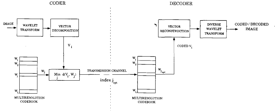
Fig. 10. Encoding/decoding scheme.
