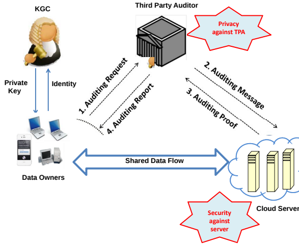
Fig. 1. The system model of identity-based RDIC
