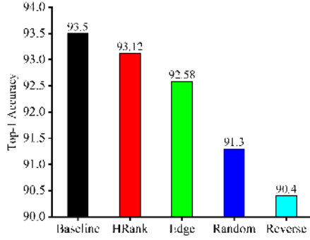
Figure 4. Top-1 accuracy for variants of HRank.
