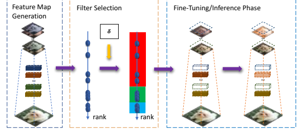
Figure 1. Framework of HRank. In the left column, we first use images to run through the convolutional layers to get the feature maps. In the middle column, we then estimate the rank of each feature map, which is used as the criteria for pruning. The right column shows the pruning (the red filters), and fine-tuning where the green filters are updated and the blue filters are frozen.
