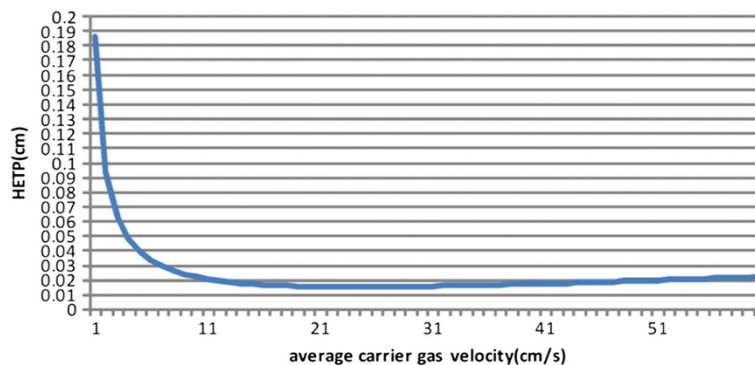
Figure 5 Height equivalent to theoretical plate ( H ) versus average carrier gas velocity for the four-capillary micro MCC. Length = 50 cm, depth = 450 μm, and width = 60 μm.
