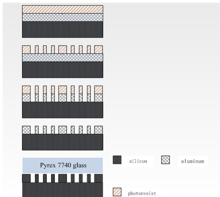
Figure 1 Multi-capillarycolumn fabrication process.
