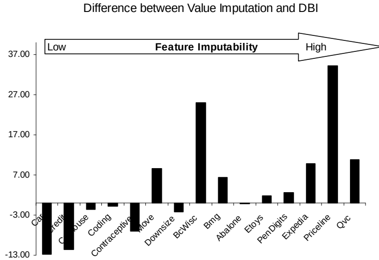
Figure 4: Differences between the relative performances of PVI and DBI. Domains are ordered left-to-right by increasing feature imputability. PVI is better for higher feature imputability, and DBI is better for lower feature imputability.
