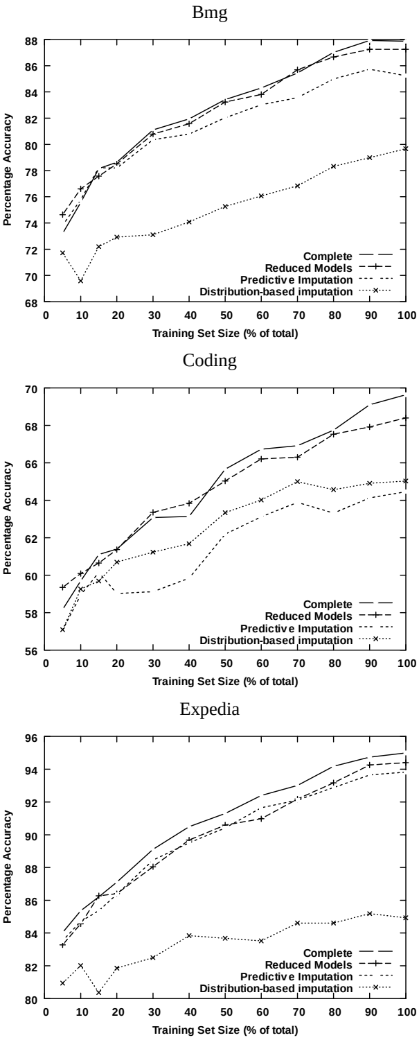
Figure 2: Learning curves for missing value treatments
