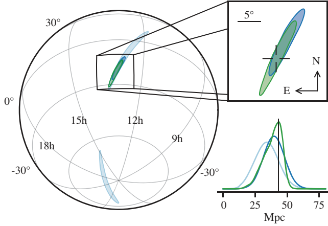
FIG. 3. Sky location reconstructed for GW170817 by a rapid localization algorithm from a Hanford-Livingston ( 190 \text{ deg}^2 , light blue contours) and Hanford-Livingston-Virgo ( 31 \text{ deg}^2 , dark blue contours) analysis. A higher latency Hanford-Livingston-Virgo analysis improved the localization ( 28 \text{ deg}^2 , green contours). In the top-right inset panel, the reticle marks the position of the apparent host galaxy NGC 4993. The bottom-right panel shows the a posteriori luminosity distance distribution from the three gravitational-wave localization analyses. The distance of NGC 4993, assuming the redshift from the NASA/IPAC Extragalactic Database [89] and standard cosmological parameters [90], is shown with a vertical line.
