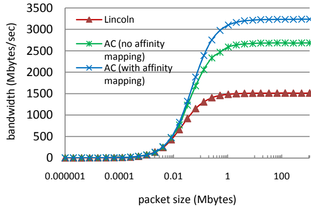
Fig. 3. Host-device bandwidth measurements for AC and Lincoln.
