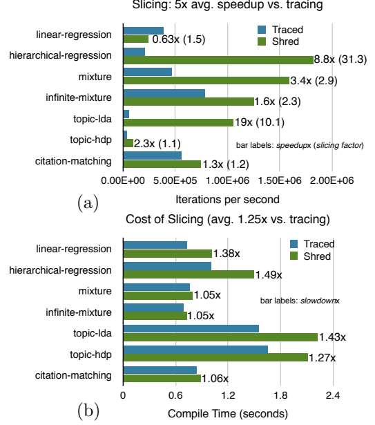
Figure 5: Effect of SHRED, our slicing-based incrementalizing scheme. (a) compares performance versus tracing and (b) compares cost in compilation time.
