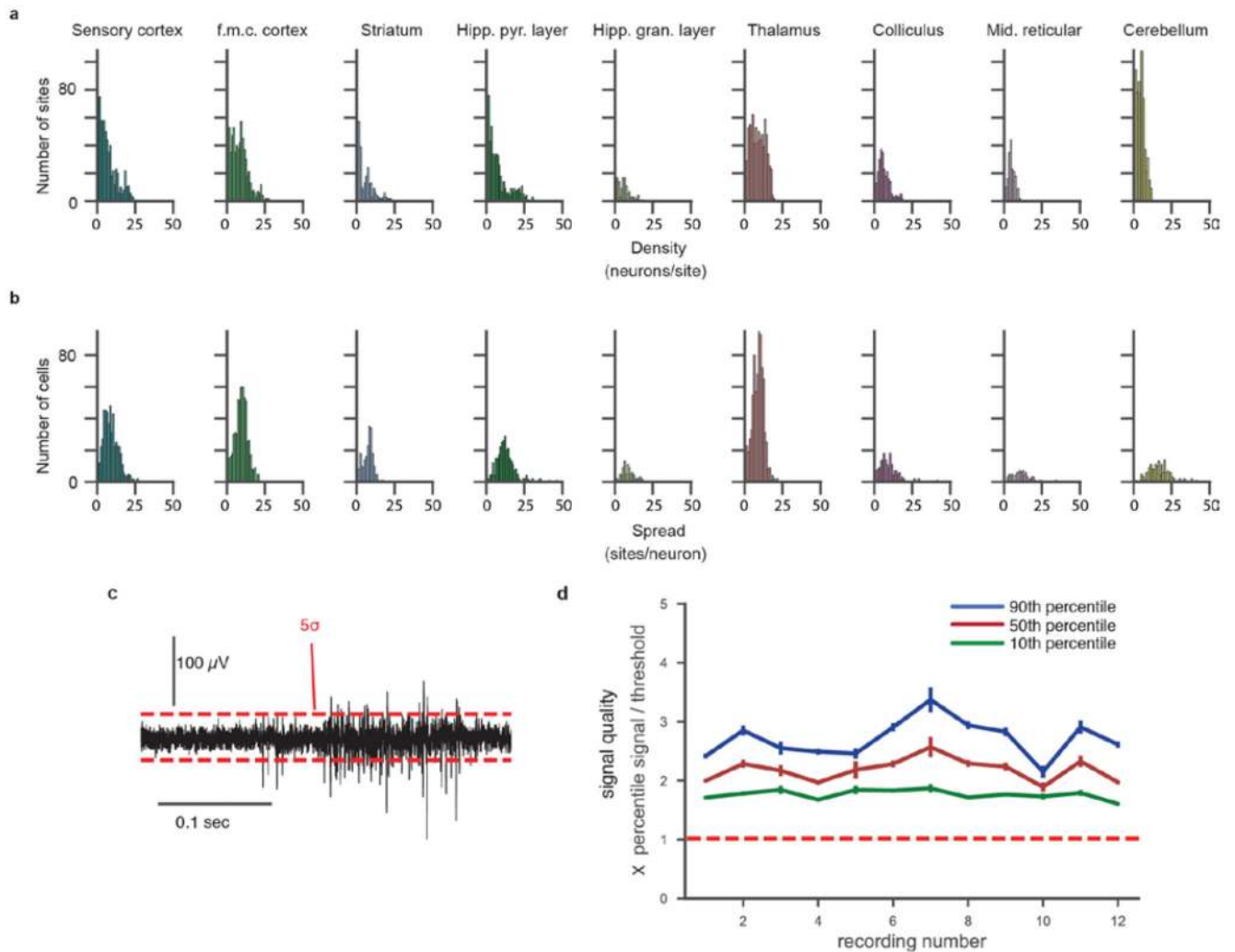
Extended Data Figure 7. Spike band signal quality across brain areas and multiple acute recordings.
