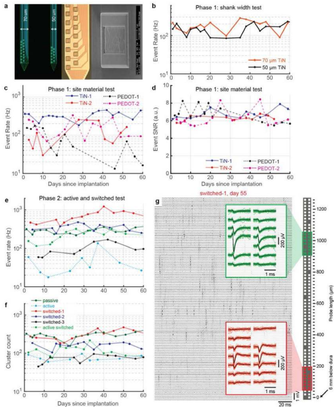
Extended Data Figure 4. Long-term stability studies: Effects of shank width, TiN sites, and active and switched sites.
