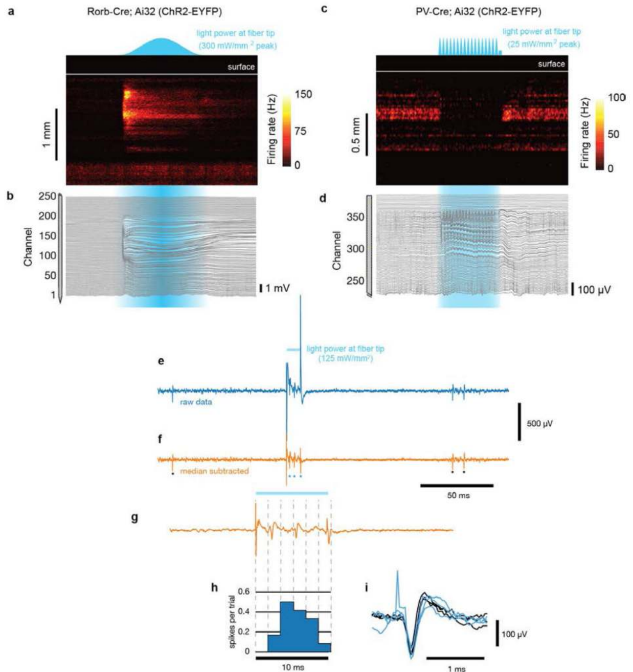
Extended Data Figure 8. Recording during optogenetic stimulation of excitatory and inhibitory cell populations.
