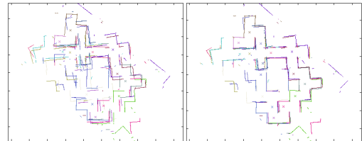
Fig. 8. Left, initial configuration of NIST's maze data (16 scans). Right, after 5 iterations of FFS.
