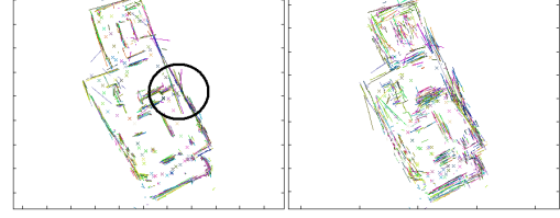
Fig. 5. Left, initial configuration of the Apartment data (91 scans). Encircled: a huge alignment error due to a loop closing effect. Right, after 5 iterations of FFS: a large step parameter \Delta_t leads to a 're-shuffling' of segments. This is needed to escape the local optimum as shown in the left configuration. Compare also the potential curve in 7
