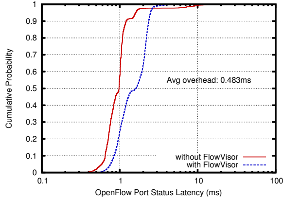
Figure 5: CDF of virtualization overhead for OpenFlow port status requests.
