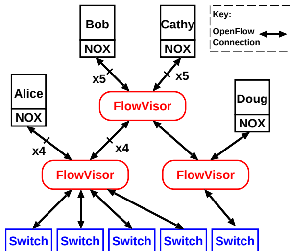
Figure 3: A single FlowVisor instance can virtualize many switches in parallel. Additionally, because of the transparent design, FlowVisor can trivially recursively slice a virtual slice, creating hierarchies of FlowVisors.
