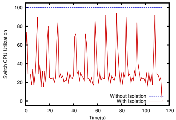
Figure 8: FlowVisor’s new flow messages throttling prevents a faulty controller from saturating switch CPU.
