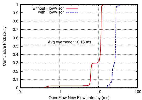
Figure 4: CDF of virtualization overhead for OpenFlow new flow messages.
