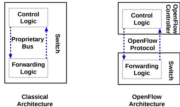
Figure 9: Relative to traditional hardware, the OpenFlow protocol moves the control path to an external controller.
