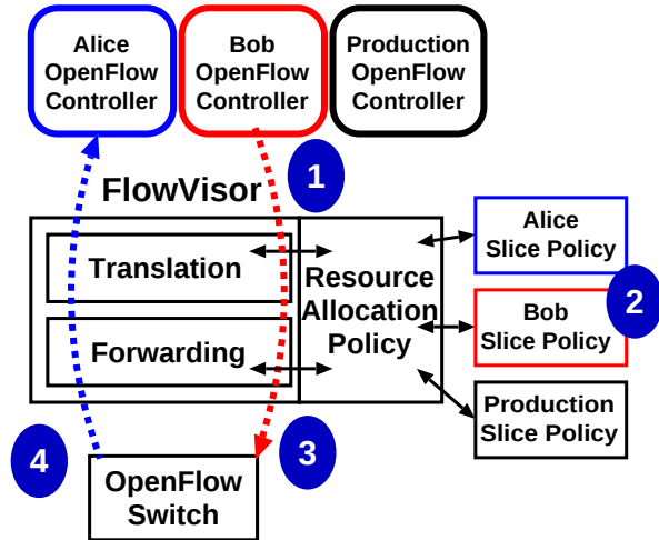
Figure 2: The FlowVisor intercepts OpenFlow messages from guest controllers (1) and, using the user’s slicing policy (2), transparently rewrites (3) the message to control only a slice of the network. Messages from switches (4) are forwarded only to guests if it matches their slice policy.
