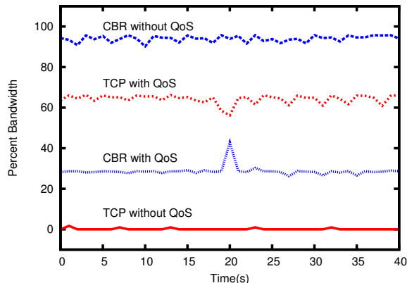
Figure 6: Effect of FlowVisor bandwidth isolation on competing TCP and CBR traffic
