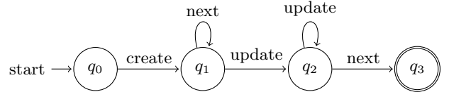
Figure 5: FailSafeIter tracematch and automaton: detect updates to a Collection which is being iterated over.
