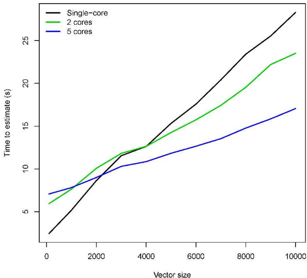
Figure 8: Potential speedup using parallelization functionality.
