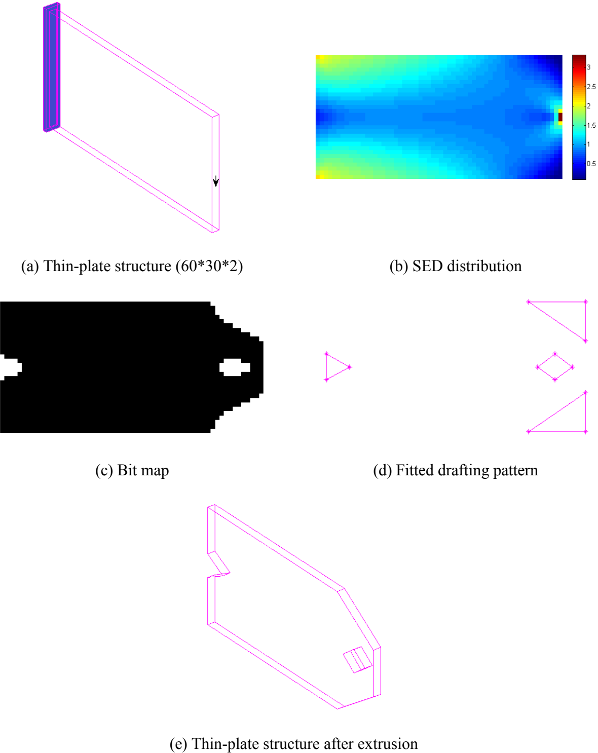
Fig. 5.6 Feature modeling process
