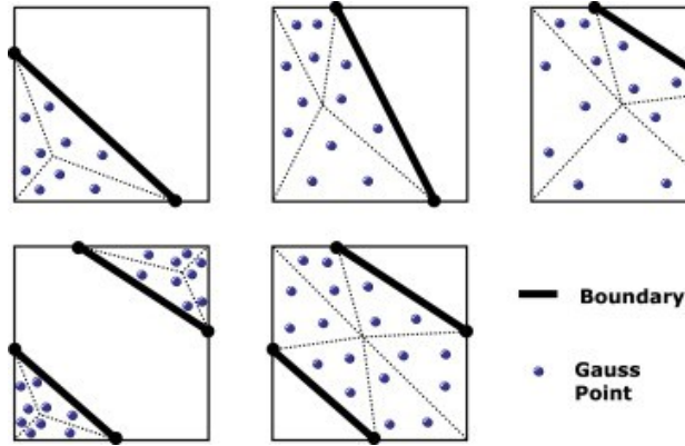
Fig. 5.2 Solid part partition of the BCEs [Wei et al. 2010]
