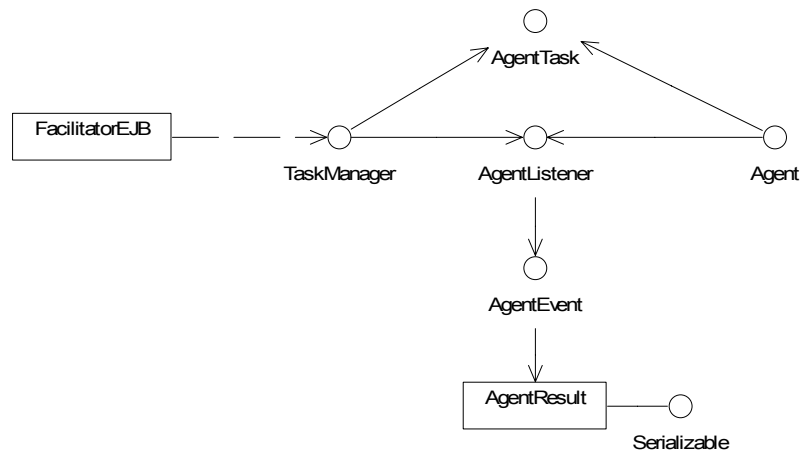
Fig. 6. Classes and interfaces used for the task execution
