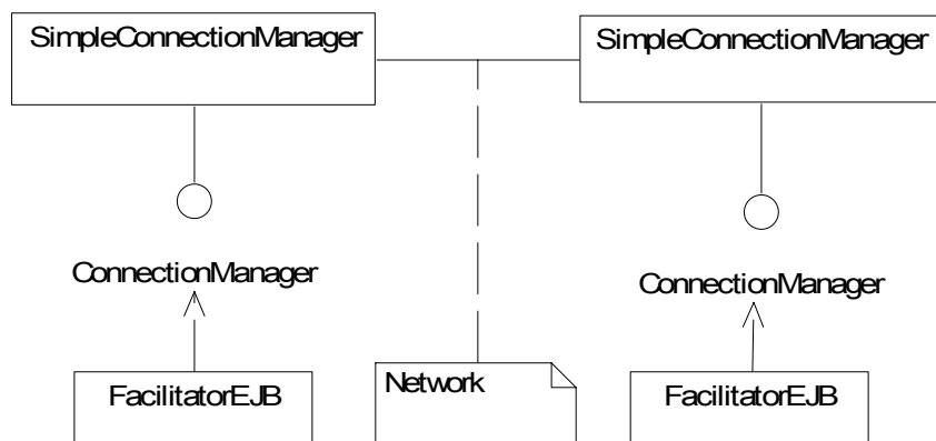
Fig. 8. ConnectionManager components provide links between frameworks
