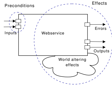
Figure 5: Plan operator representation of a web service.
