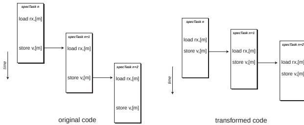
Example 2 - Moving a loop carried dependency to improve method speculation performance.
