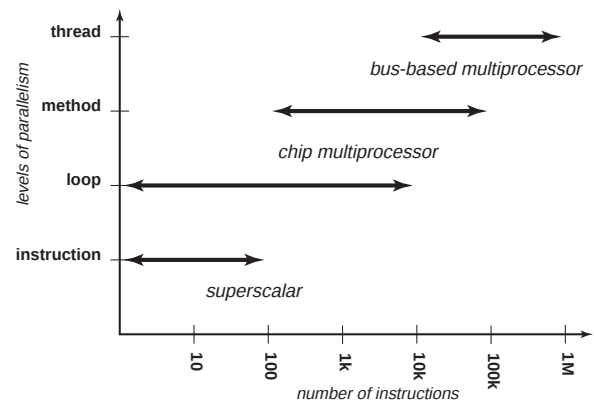
Figure 1 - A single chip multiprocessor can exploit levels of parallelism not available to traditional superscalar processors or bus-based multiprocessors.
