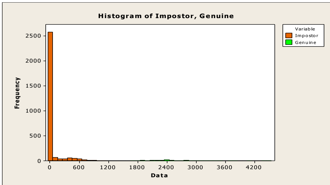
Figure 2.2 Score histogram
