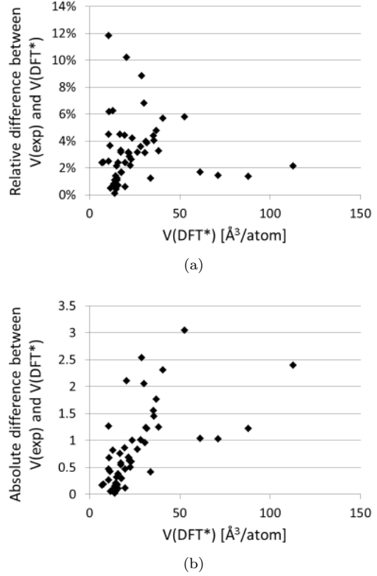
Figure 4. Relative (a) and absolute (b) differences of the DFT regression data (DFT*) with respect to thermally corrected experimental values [43, 76–83] for the equilibrium volume
