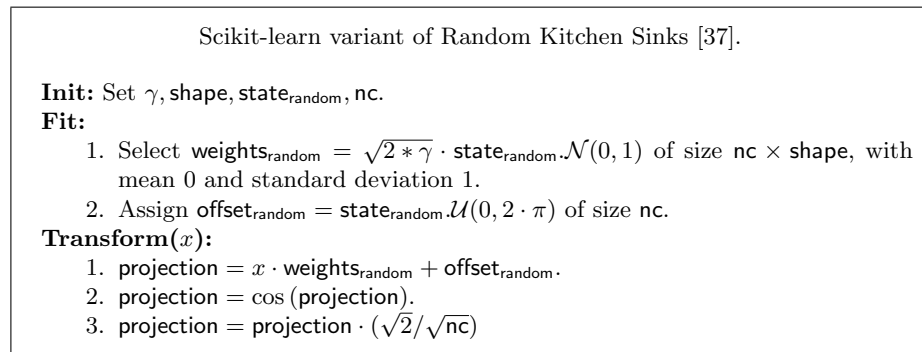
Fig. 2. RBF Sampler.
