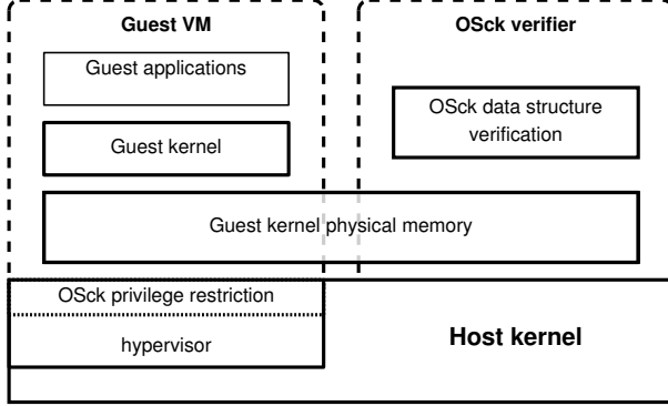
Figure 3. OSck architecture. Most of OSck’s verification runs in a thread at the same privilege level as the guest OS, isolated by process and VM boundaries.
