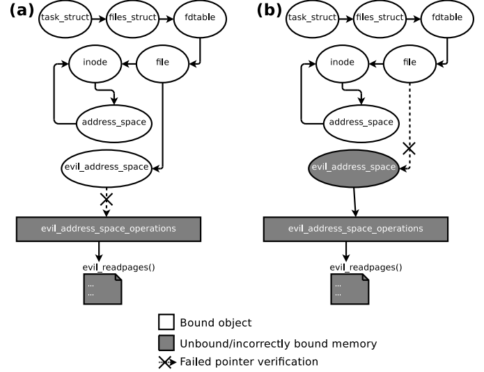
Figure 5. Modified type graph created by a malicious modification to the kernel heap, with two possible bindings from object to type. Regardless of binding, malicious modification will cause verification to fail.
