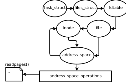
Figure 4. A subset of the kernel type graph. The kernel’s traversal of this graph will result in the execution of the safe function readpages .
