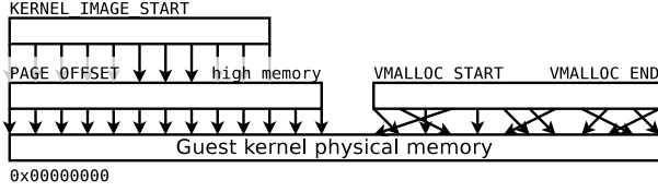
Figure 6. Mapping guest OS memory into the OSck verifier address space.
