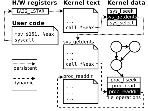
Figure 1. Control transfers in kernel invocation of a getdents system call. Static control transfers occur within blocks of kernel text. Persistent and dynamic control transfers use values in hardware registers and kernel memory to determine the next instruction executed.
