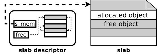
Figure 7. Slab organization of kernel memory allocations. Information about allocated and free objects within a slab is contained in a slab descriptor’s internal list.
