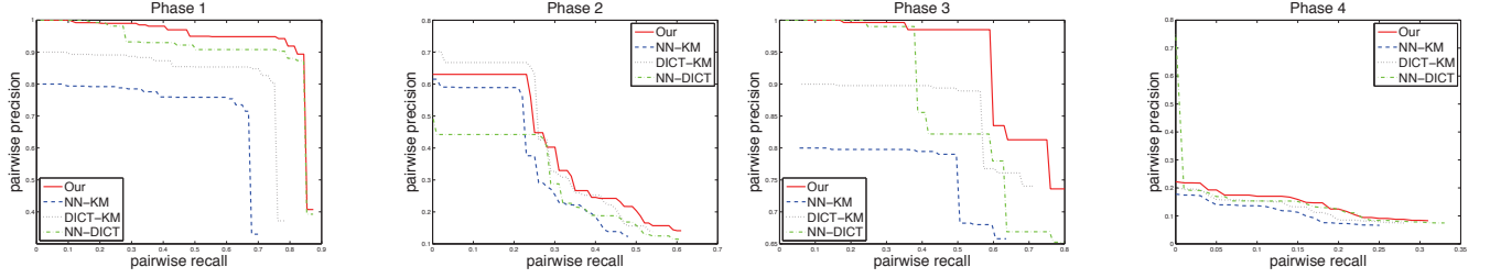
Figure 4: Interpolated pairwise precision-recall curves for TDT2, obtained by varying \zeta and \eta between [0.05, 0.15] .
