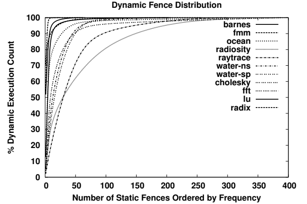
Figure 8: Distribution of fences
