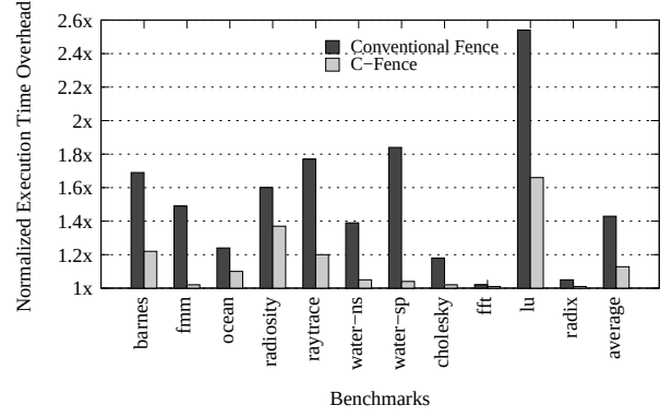
Figure 11: Execution time overhead of ensuring SC: Conventional fence vs C-Fence.
