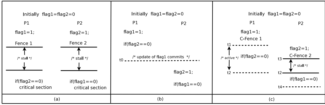
Figure 3: (a) SC using memory fences. (b) Scenario in which fences are not required. (c) SC using conditional fences.
