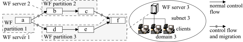
Fig. 2. Partitioning of a WF graph and distributed WF execution
