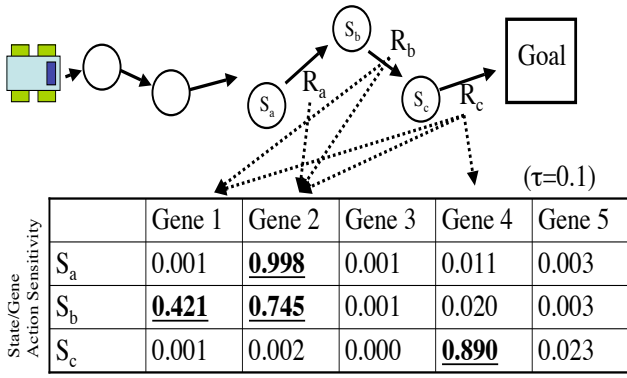
Figure 2: Action Sensitivity. A rover with a policy defined by 5 genes moves through different states to a reach a goal. Action sensitivities seen in the final three states shown in the table. Only Gene 2 influences rover’s action in state S_a above the threshold \tau so it is the only gene that gets credit for reward R_a . Genes 1 and 2 influence rover’s action in state S_b so both get credit for R_b . Gene 4 influences rover’s action in state S_c so it gets credit for R_c . Since the actions taken at states S_a and S_b are responsible for the rover entering state S_c , the reward R_c must also be propagated back to Gene 1 and 2 for their contributions.
