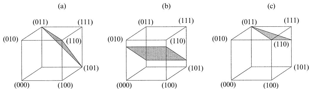
Fig. 2. Geometric representation of rounding problem. (a) shows fixed size constraint when all the vertices of K are vertices of the cube. In (b) none of vertices of K is a vertex of the cube. In (c) some vertices of K are vertices of the cube and others are not.
