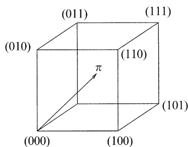
Fig. 1. Geometric representation of possible samples in a population of size N = 3 .
